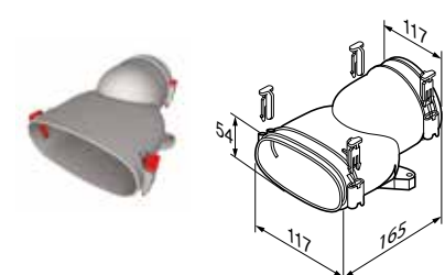
Figure 1. 90° bend
