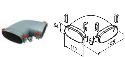
Figure 2. 90° Lateral bend
