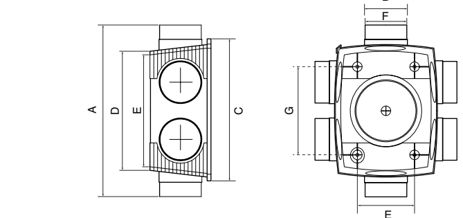
Rear box dimensions for WHV8/6, WHV8R/6, HVS10/6, HVS10R/6
