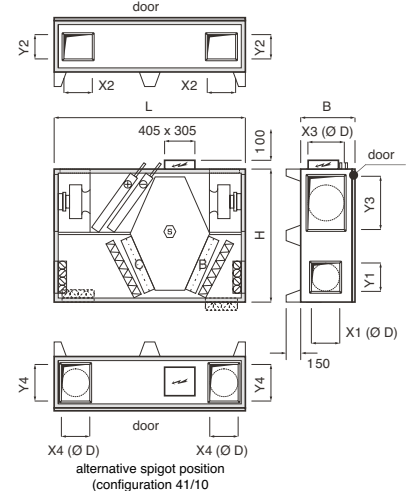
FLOOR STANDING FLAT (top view) Multi DV500 to DV6500 alternative spigot position (configuration 41/5)
