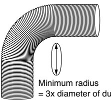
Figure 2. 90° Lateral bend
